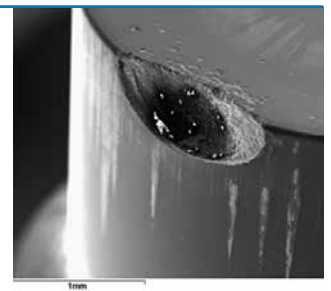
Edge chipping due to cyclic plastic deformation
