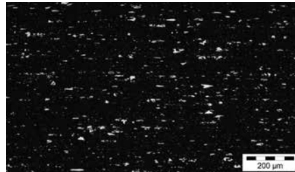
Microstructure of 8% chromium steel in ESR grade
